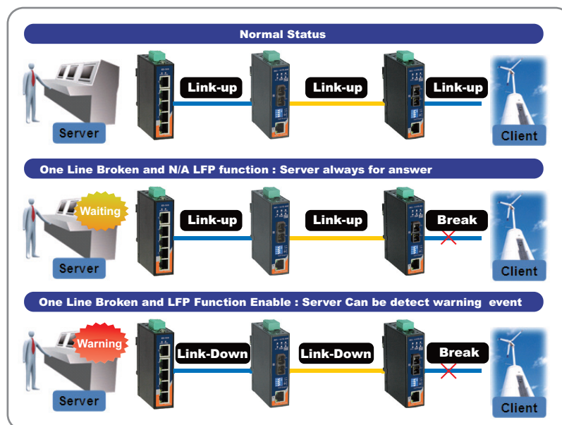
Connections of Media Converter and LFP function
