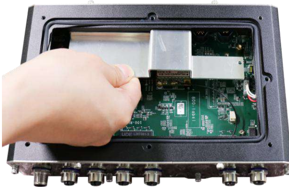
Place heatsink back on the modules
