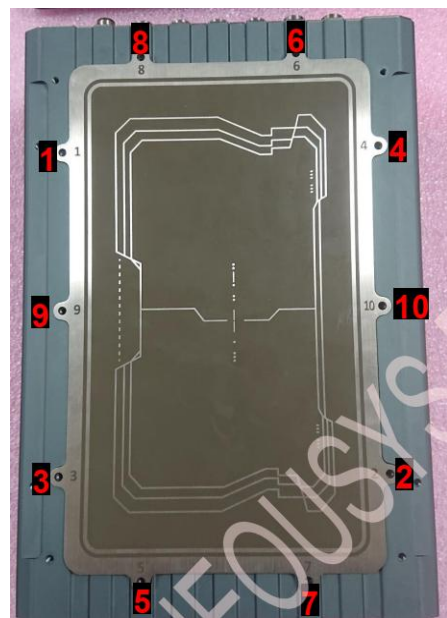
Attach the backplate, incremental screw order, and at a specified torque range (8.1 – 9.9kgf-cm)
